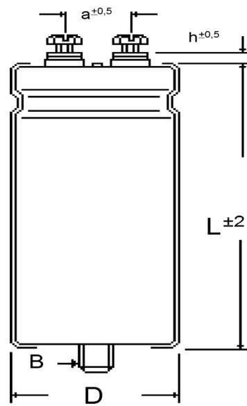
Fig2: GHB for stud mounting
